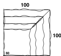
ANGLE EL.
