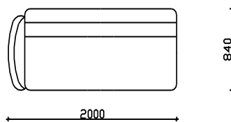
ANGLE 3 SEATER
